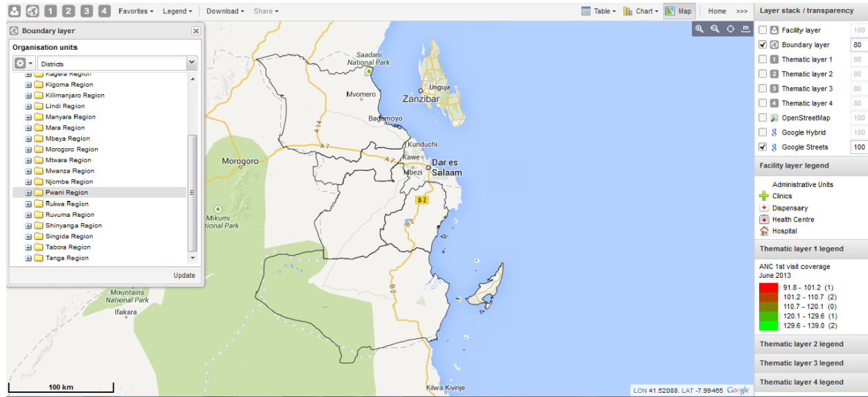
Figure 7.4: Boundary Layer Parameters
